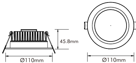
Cut-out: Ø90mm-100mm
