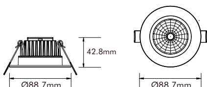
Cut-out: Ø68mm-75mm
