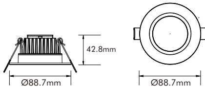
Cut-out: Ø68mm-75mm
